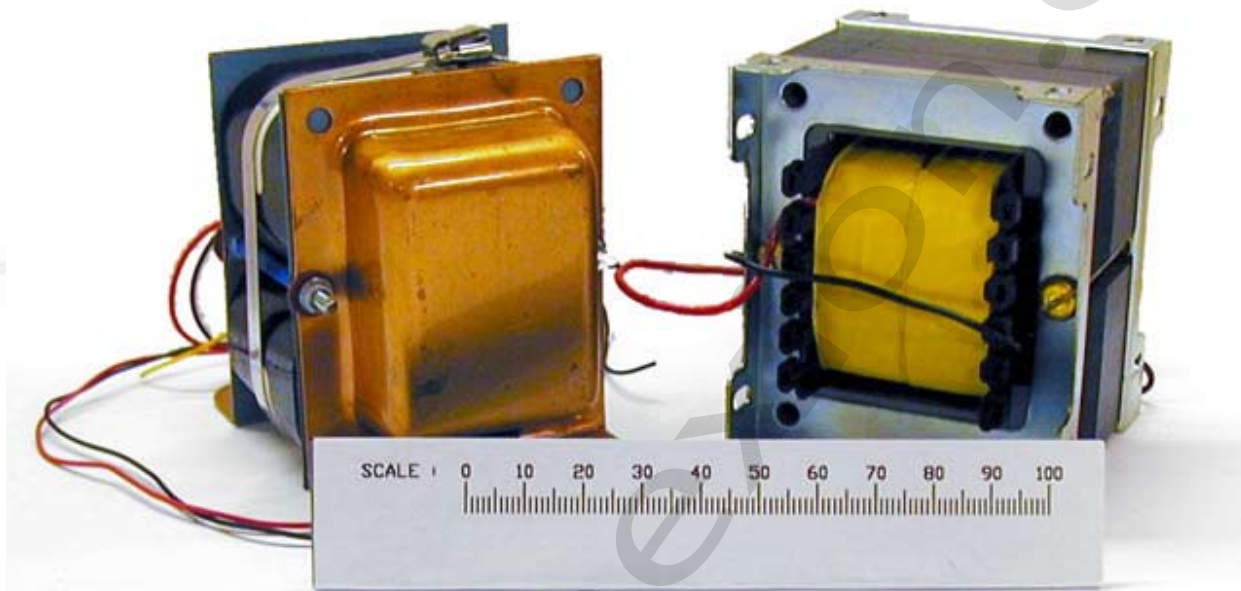
TRANS-027/03-C (TXP-028-3-55-ANPT-ANPT-SC) in optional copper shrouds & TRANS-011 (TXP-011) in standard steel frames
